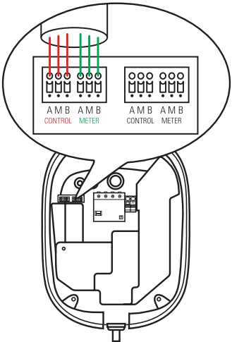
Slave - Address 2
