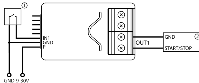
Diagram 9: Example gate opener
