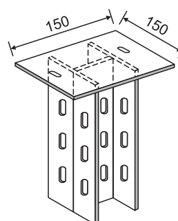
Flanged Double U - Channel Piece
