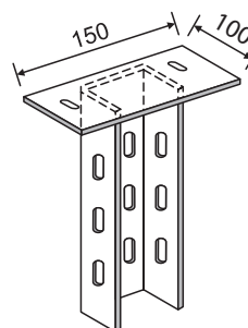
Flanged U - Channel Piece
