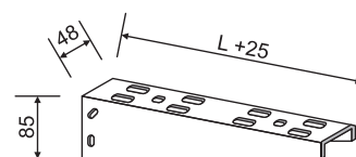
Brackets
