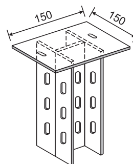
Flanged Double U - Channel Piece
